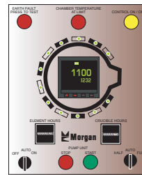
Control panel. ▲
